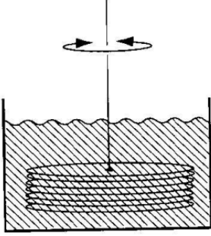
Figure 2.11: The Andronikoshvili experiment. Since normal fluid sticks between the closely spaced disks (but superfluid does not), the moment of inertia of the stack of disks, and hence frequency of oscillation of the disks tells us the fraction of fluid that is superfluid.
