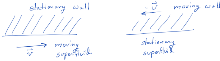
Figure 2.9: Left: Flowing a fluid past a wall. Right: In the fluid frame, the wall is moving.
