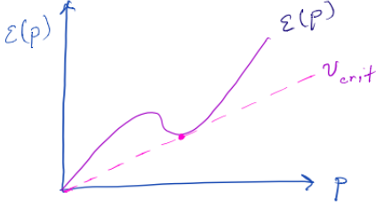
Figure 2.10: A spectrum \epsilon(p) and the corresponding critical velocity for the superfluid.
