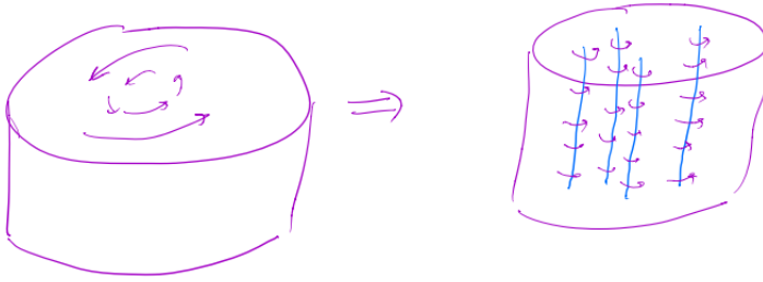
Figure 2.8: If we start a bucket of helium rotating above the critical temperature and then we cool it below the critical temperature, the circulation is accommodated by the introduction of many vortex lines.
