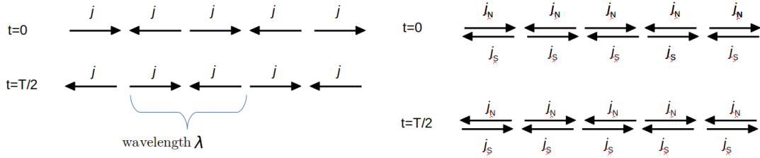
Figure 2.6: Left: Sound waves are density waves: mass sloshes back and forth. Right: Second sound waves involves counterflow. There is no mass transport, although heat is transported.
