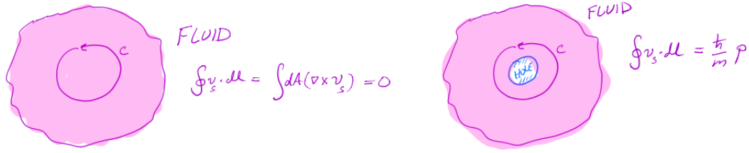
Figure 2.7: Left: A contour in fluid that can be contracted and therefore bounds a disk in the fluid. In this case the circulation must be zero. Right: A contour in fluid that cannot be contracted. In this case we can only say that the circulation is quantized in units of the elementary circulation quantum h/m .
