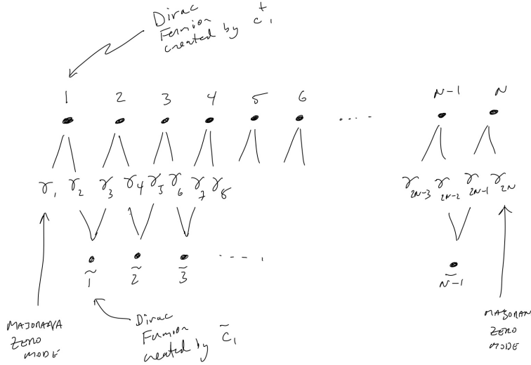
Figure 12.2: Here how the Kitaev chain takes a system of Dirac fermions (top), splits them into Majoranas (middle) and then regroups them into new Dirac fermions (bottom) leaving one Majorana zero mode at each end of the chain.
