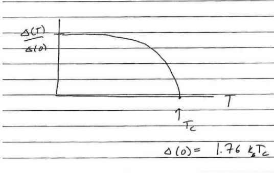
Figure 11.5: Gap as a function of T
