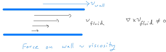
Figure 2.3: The standard experiment to measure viscosity requires vorticity.
