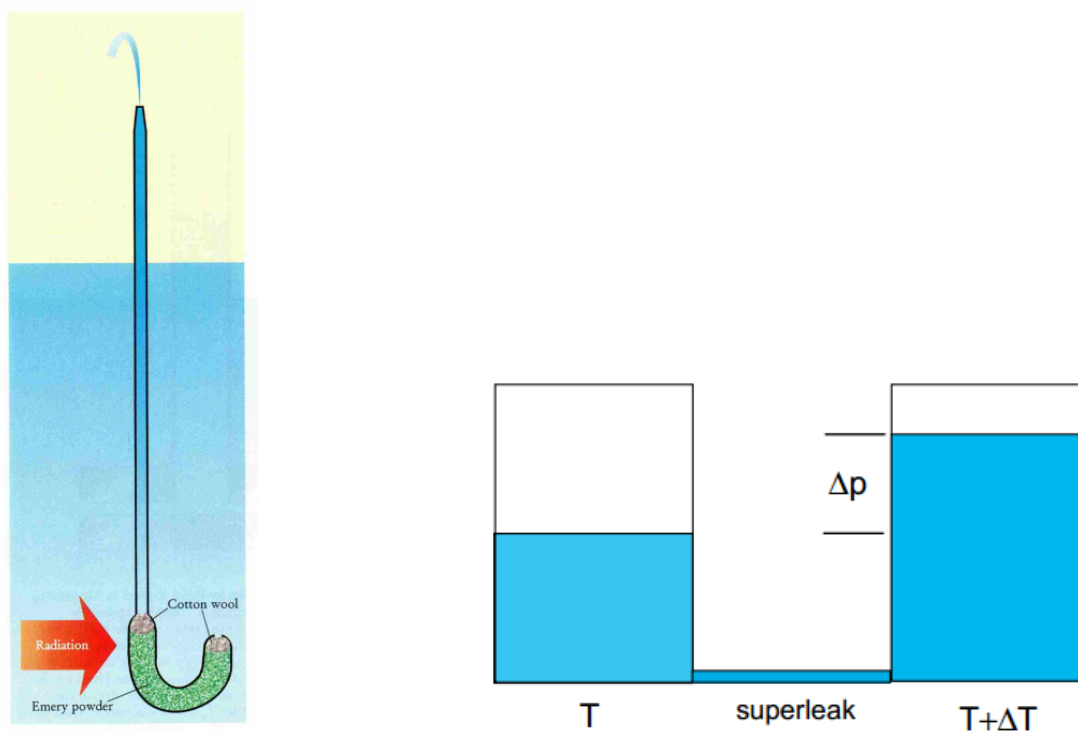
Figure 2.4: Left: The fountain effect. A tube is inserted in the superfluid and plugged with cotton such that only the “super” fraction of the fluid can get through. Heating the cotton, will result in superfluid being sucked into the tube at a high rate such that it can fountain out the top. Right: a similar experiment showing that a temperature difference implies a pressure difference.
