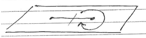
Figure 12.4: Dragging a vortex around one end of the wire the wire rotates the phase by 2\pi at one end of the wire, but does not rotate the phase at the other end of the wire. This implements an X gate on the qubit.
