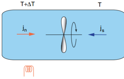
Figure 2.5: Thermomechanical Effect: The propeller turns as if fluid is flowing from hot to cold, even though there is no net transport of mass.
