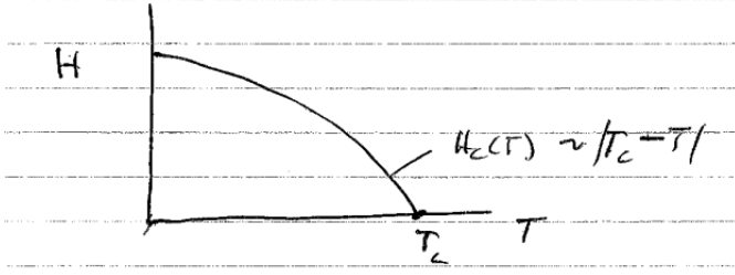
Figure 6.4: The critical field scales linearly with T - T_c close to T_c , at least within a mean field theory calculation.
