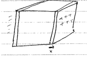
Figure 8.6: Displacing all of the mobile charges by a distance x builds up a surface charge \rho_{\text{surface}} = \bar{n}xe
