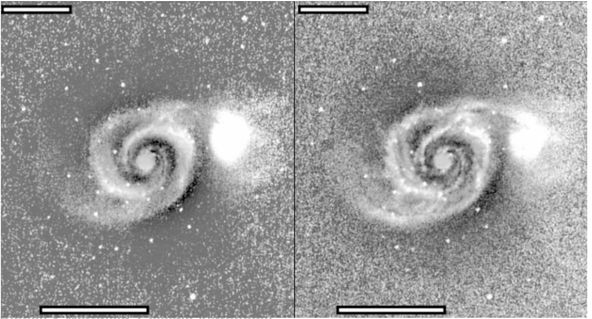
Binney & Merrifield, Galactic Astronomy
