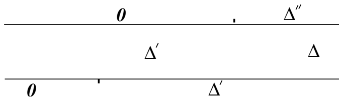
Figure 13: Argument illustrating the fusion rules.
