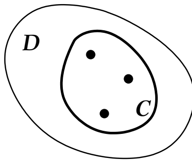
Figure 1: We consider an infinitesimal transformation which is conformal within C and the identity in the complement in \mathcal{D} .
