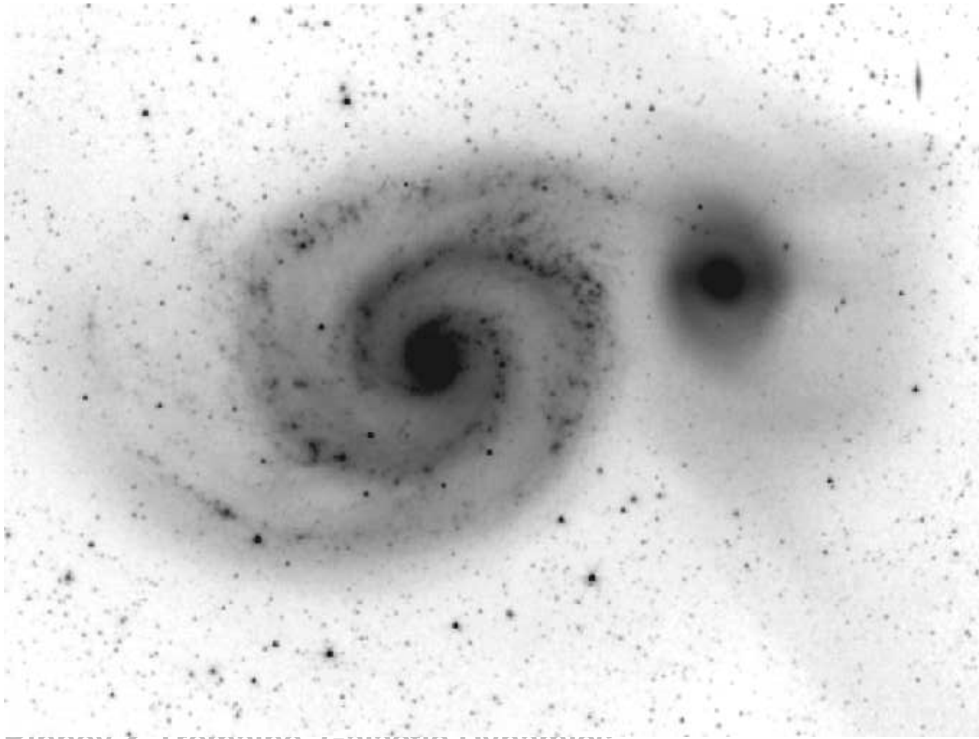
Binney & Tremaine, Galactic Dynamics
