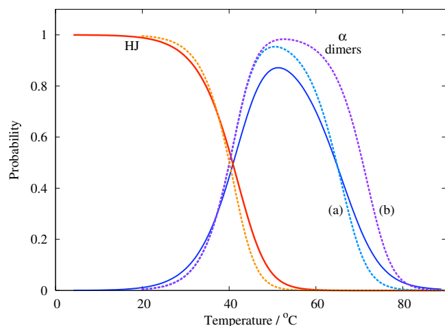
FIG. 12. (Color online) Bulk equilibrium probability of strands being in a Holliday junction or an \alpha -bonded dimer computed by umbrella sampling (solid lines) and by the ETSM (dashed lines), where lines (a) and (b) represent the two possible \alpha -bonded dimers.
