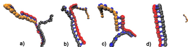
FIG. 6. (Color online) Snapshots illustrating four stages in the process of displacement. (a) A third strand binds to a misbonded pair. (b) The third strand is prevented from forming a complete duplex by the misbond. (c) Thermal fluctuations cause bonds in the misbonded structure to break and be replaced by the correct duplex. (d) The misbonded strand is displaced and the correct duplex is formed.
