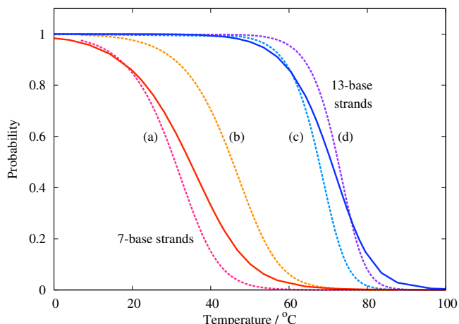
FIG. 5. (Color online) The bulk equilibrium probability of strands being in a correct duplex extrapolated from our umbrella sampling simulations (solid lines) compared to the predictions of an empirical two-state model (dashed lines). Results are presented for strands with 7 and 13 bases, as labeled. For the two-state model, as well as the results for the sequences in Eqs. (7) and (8) [lines (a) and (d)], sequences corresponding to the other two arms of the Holliday junction (Fig. 7) are considered. Only one line is shown for the umbrella sampling results, because A-T and G-C have the same binding energy in our model. Temperatures in our model are converted to ^{\circ}C using the mapping given in Sec. II A.
