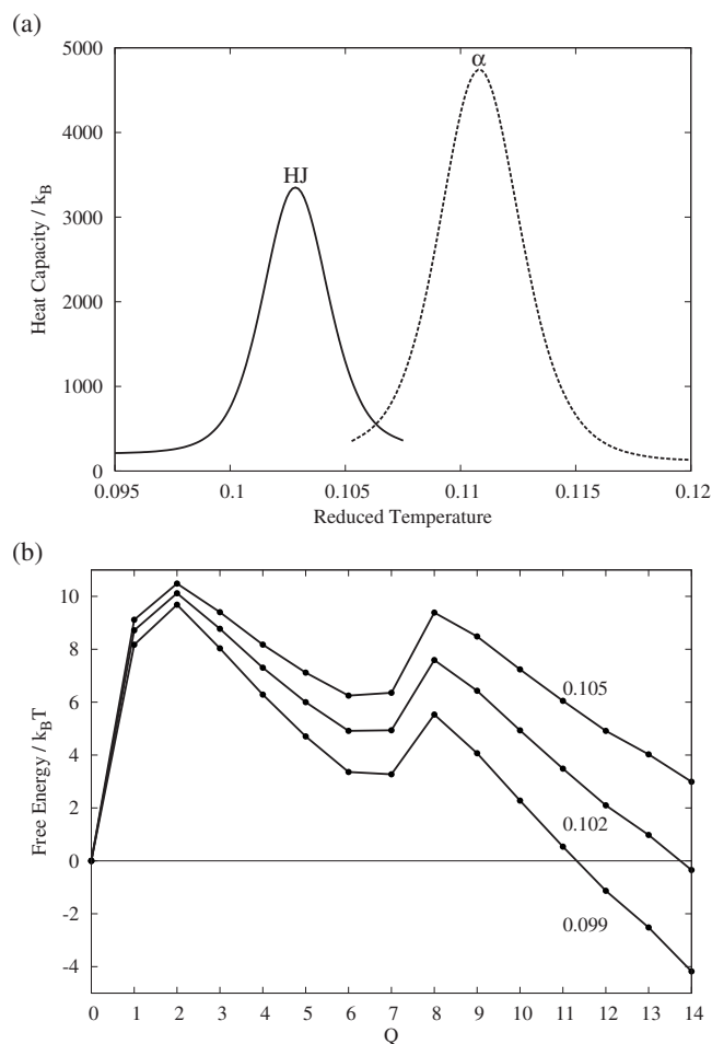
FIG. 11. Thermodynamics for the formation of a single Holliday junction. (a) Heat capacity curves for two \alpha -bonded dimers forming a Holliday junction and four strands forming two \alpha -bonded dimers, as labeled. (b) Free energy profiles for the formation of a Holliday junction from two \alpha -bonded dimers at different temperatures, as labeled. Q represents the total number of correct bonds in the short arms of the junction.
