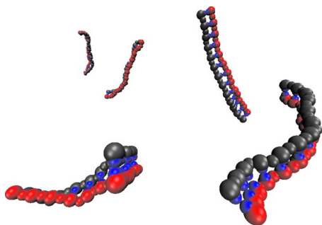
FIG. 3. (Color online) Snapshot of a fully assembled configuration in a MC simulation of ten 13-base strands at T^*=0.0971 . Backbone sites are indicated by the large spheres, and bases by smaller spheres.
