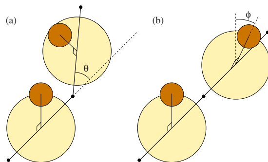
FIG. 1. (Color online) A schematic representation of the model. The thick lines represent the rigid backbone monomer units and the large circles represent the repulsive LJ interactions at their centers. The smaller, darker circles represent the bases. The panels illustrate the definitions of (a) the bending angle between two units ( \theta ) and (b) the torsional angle ( \phi ) which is found after the monomers have been rotated to lie parallel.
