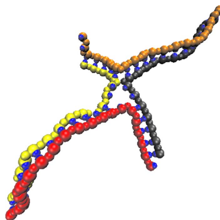
FIG. 14. (Color online) Example of a competing minimum for a badly designed Holliday junction. The snapshot is taken from a simulation at T^* = 0.0936 .
