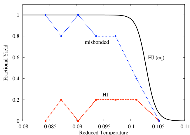
FIG. 13. (Color online) Simulation results for the badly designed Holliday junction of Sec. III C, where the initial configuration was a pair of \alpha -bonded dimers. The lines with data points give the yield of correctly formed junctions and misbonded configurations, as labeled. For comparison, the solid line gives the equilibrium probability that the well-designed sequences of Section III B adopt a Holliday junction.
