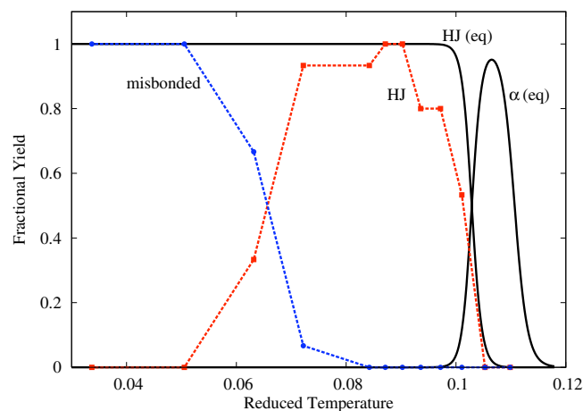
FIG. 10. (Color online) The yields of Holliday junctions and misbonded configurations for MC simulations, where the initial configuration was a pair of \alpha -bonded dimers. For comparison, the equilibrium probabilities of being in an \alpha -bonded dimer and a Holliday junction are also plotted. The results are averages over fifteen runs of length 7.5 \times 10^8 steps per strand.
