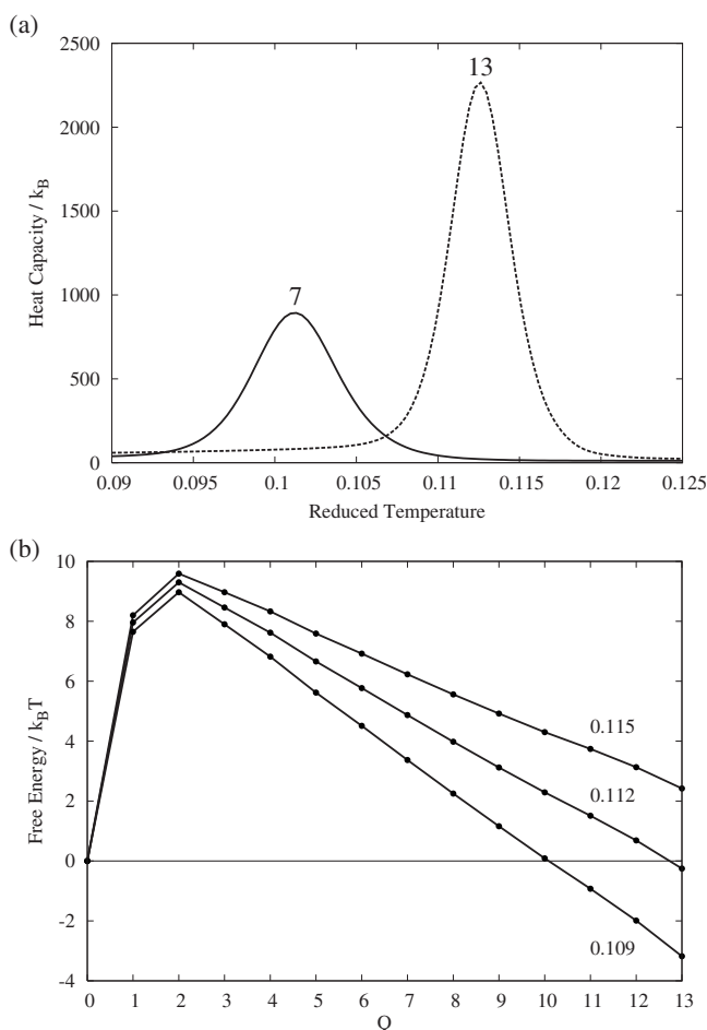
FIG. 4. Thermodynamics for the formation of a single duplex. (a) Heat capacity curves for 7- and 13-base systems, as labeled. (b) Free energy profile associated with the formation of a 13-base pair duplex at different temperatures (as labeled), where Q represents the number of correctly formed bonds in the duplex.
