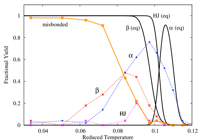
FIG. 8. (Color online) A comparison of the kinetics and thermodynamics for a system of 20 strands that can potentially form five Holliday junctions, where the MC simulations are initiated from a purely single-stranded configuration. The MC results (lines with data points) are the final yield of Holliday junctions, and the fraction of strands involved in a correctly formed long ( \alpha ) or short ( \beta ) arm, or in misbonding, as labeled. The results are averages over five runs of length 10^9 steps per strand. For comparison, the equilibrium probabilities of being in an \alpha -bonded dimer and a Holliday junction are also plotted, along with the equilibrium probability of being in a \beta -bonded dimer if the longer arms are not allowed to hybridize.
