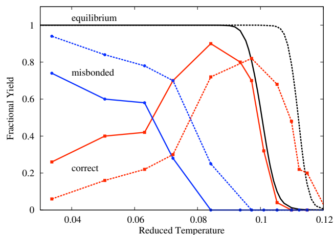
FIG. 2. (Color online) Yields of correctly formed duplexes and misbonded configurations at the end of our MC simulations (lines with data points, as labeled) compared to the equilibrium probability of the strands adopting the correct structure as obtained by umbrella sampling. The solid and dashed lines represent the results for strands with 7 and 13 monomers, respectively. The MC results are averages over ten runs of length 3 \times 10^8 steps per strand with ten strands in the simulation cell.
